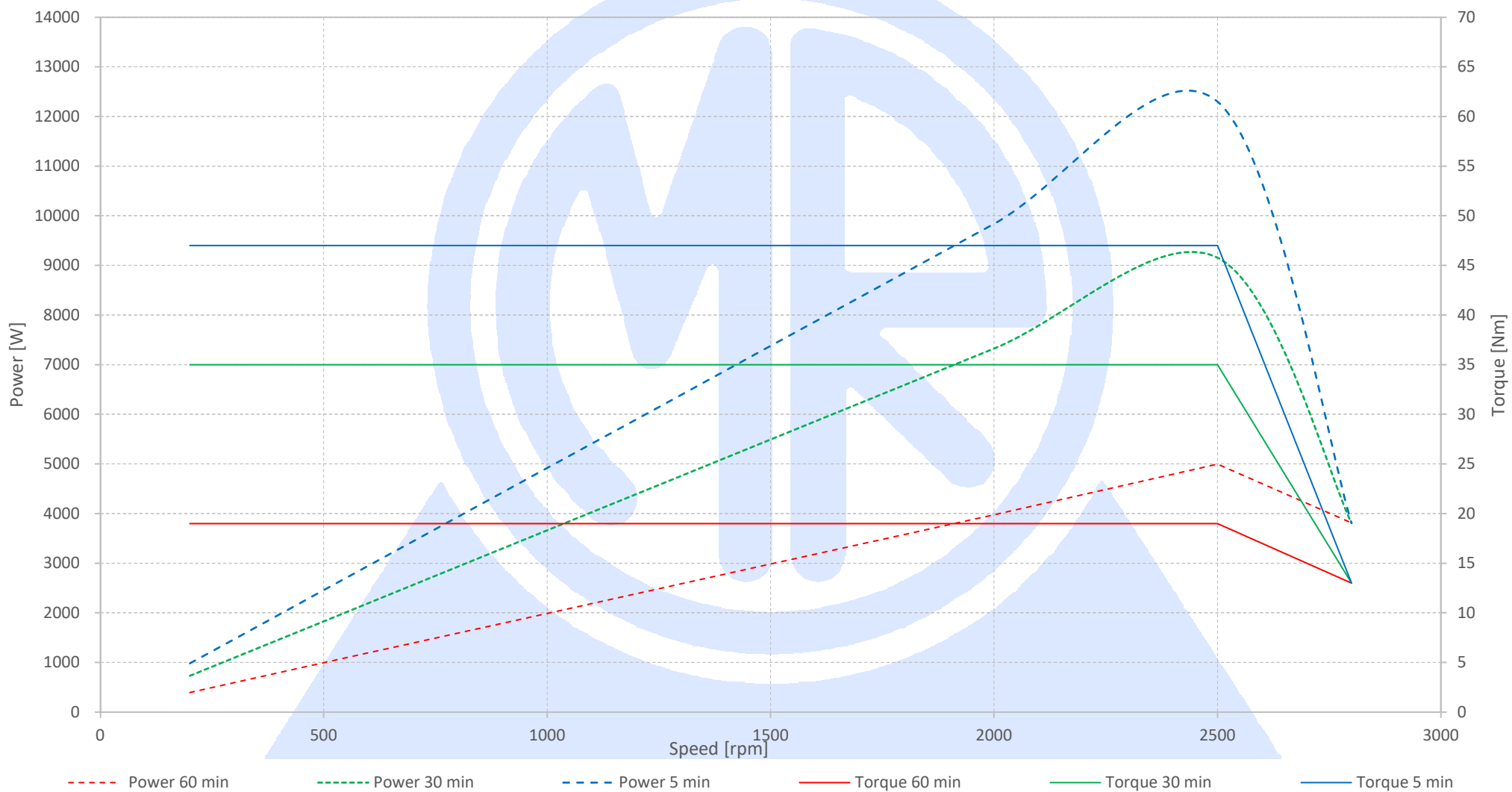
Duty Cycle Curve PSFBL101
